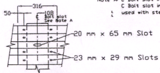
ELEVATION RAIL ELEMENT SPLICE DETAIL
