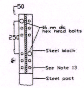
DETAIL A STEEL BLOCK ATTACHMENT TO STEEL POST
