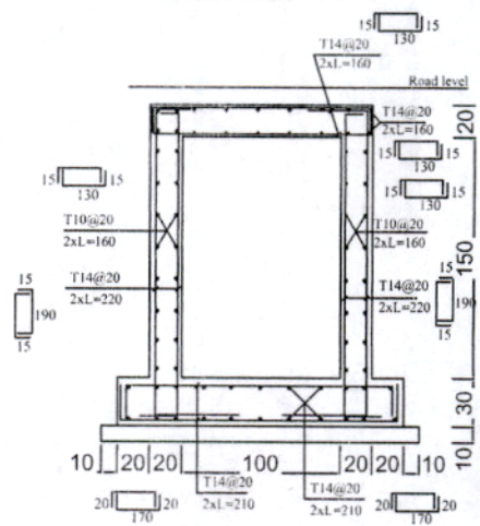
SECTION C-C
