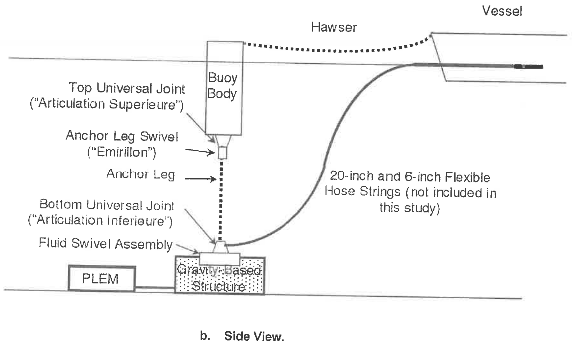
Figure 1: Field Layout of Zouk SPM Terminal.
