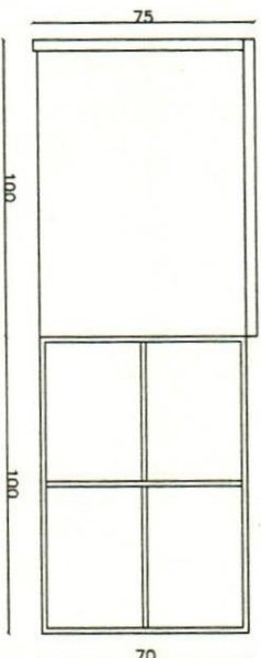
Side Elevation
