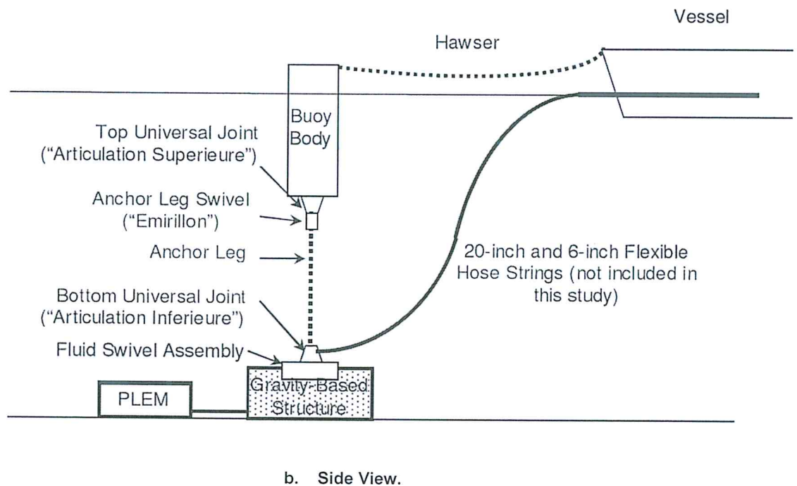
Figure 1: Field Layout of Zouk SPM Terminal.
