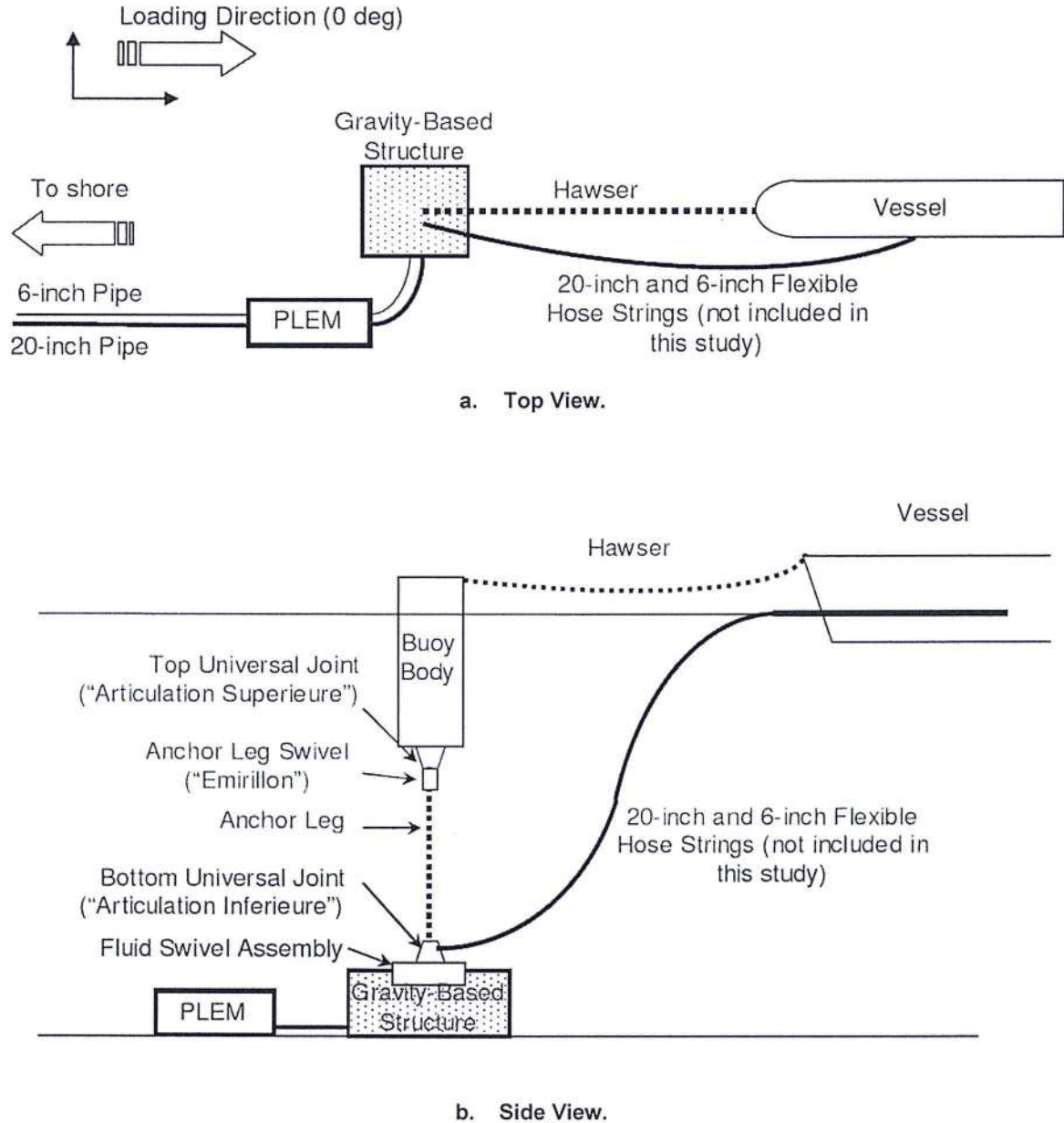
Figure 1: Field Layout of Zouk SPM Terminal.
